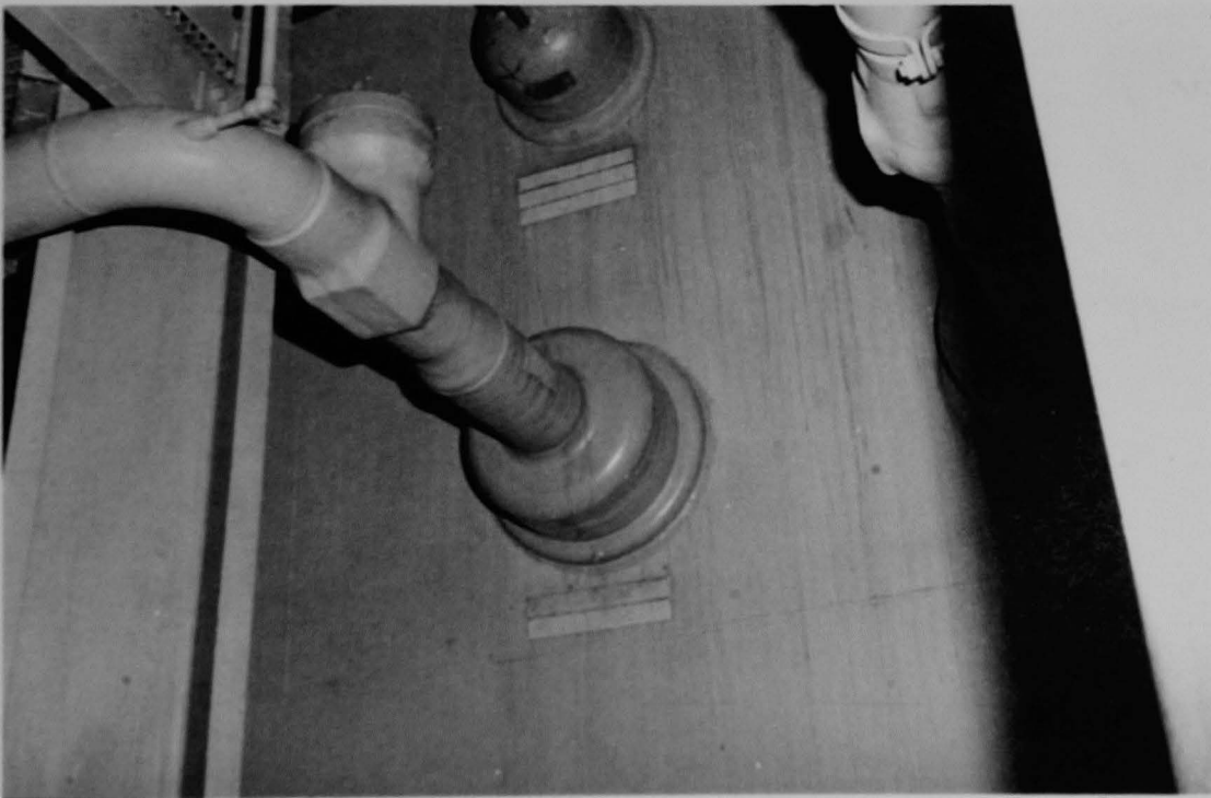
Figure 87 (5A). Mechanical penetrations R-563 and R-567 on the containment wall.
