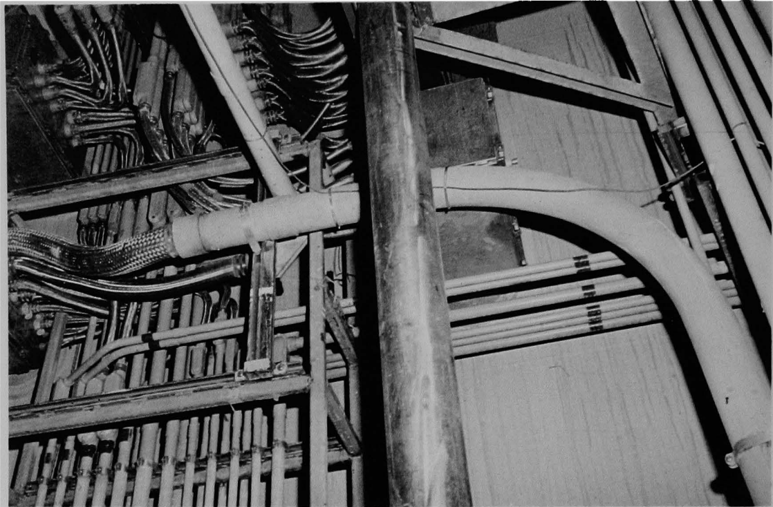
Figure 76 (5A). Electrical penetrations on containment liner (continuation to the left and lower of Figure 75).
