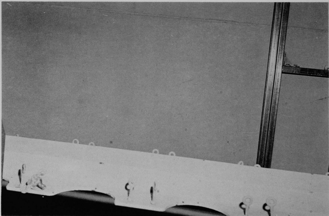
Figure 153 (6A). A top portion of the reactor vessel stud storage stand.
