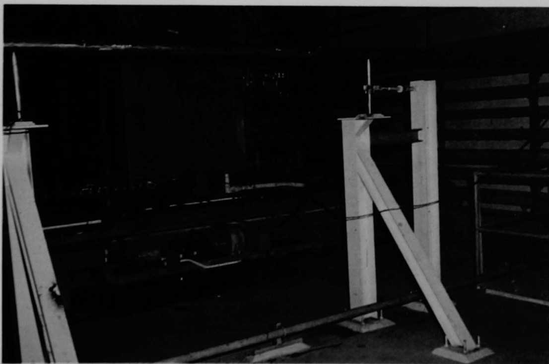
Figure 222 (4A). Power track and bridge motor of auxiliary fuel handling bridge.
