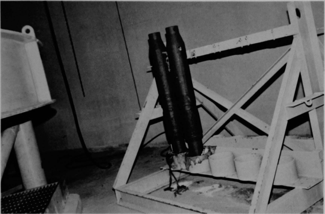
Figure 150 (2B). Storage stand for the reactor vessel studs.
