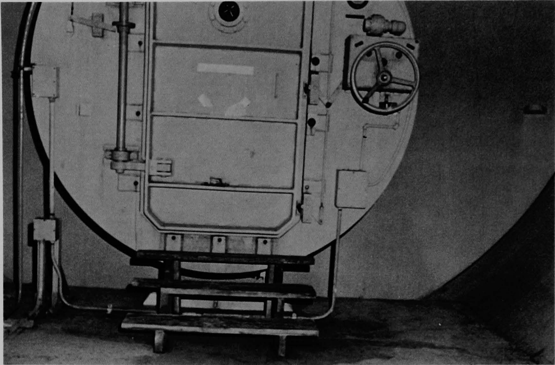
Figure 50 (1A). Personnel air lock 1, within equipment hatch.
