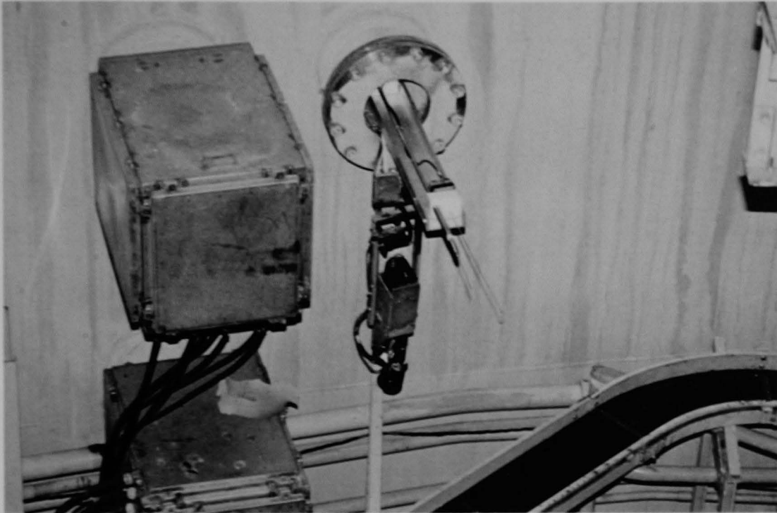
Figure 175 (4B). Penetration 626, with video camera and telemeter dosimetry antennas.
