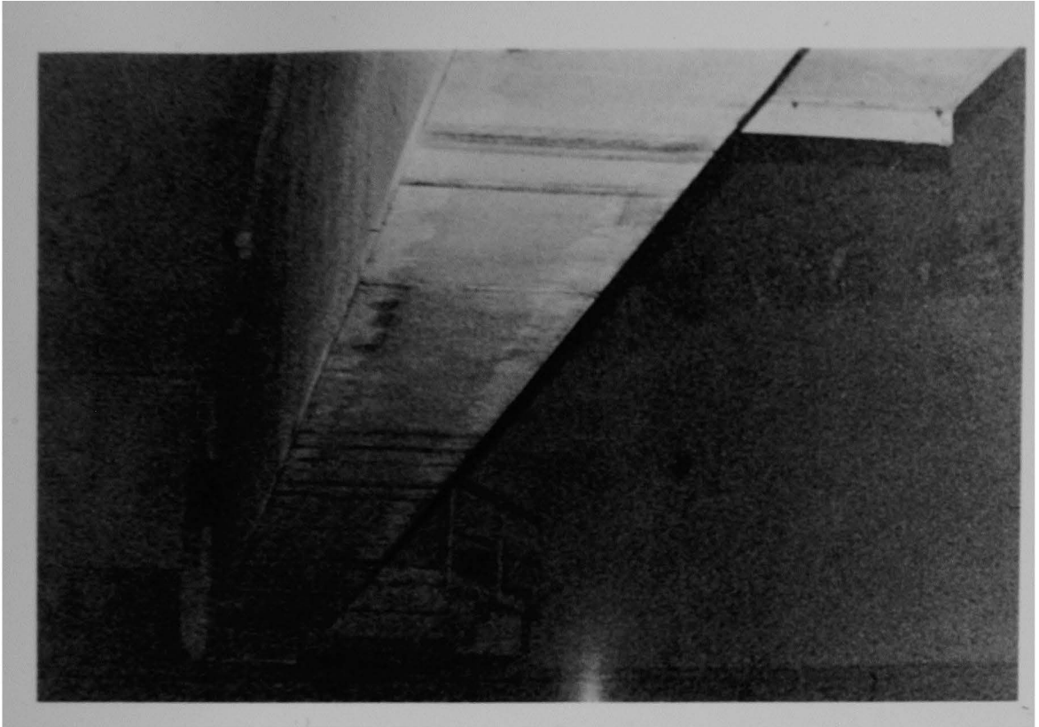
Figure 308 (5B). View northwest across containment down the length of girder B of the polar crane.
