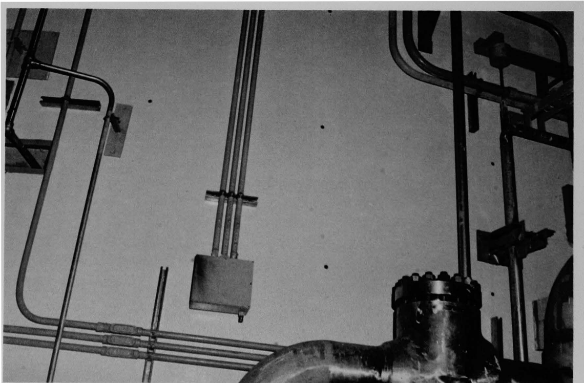
Figure 59 (2A). Circuit box, core flood B check valve, and piping along D-ring wall.
