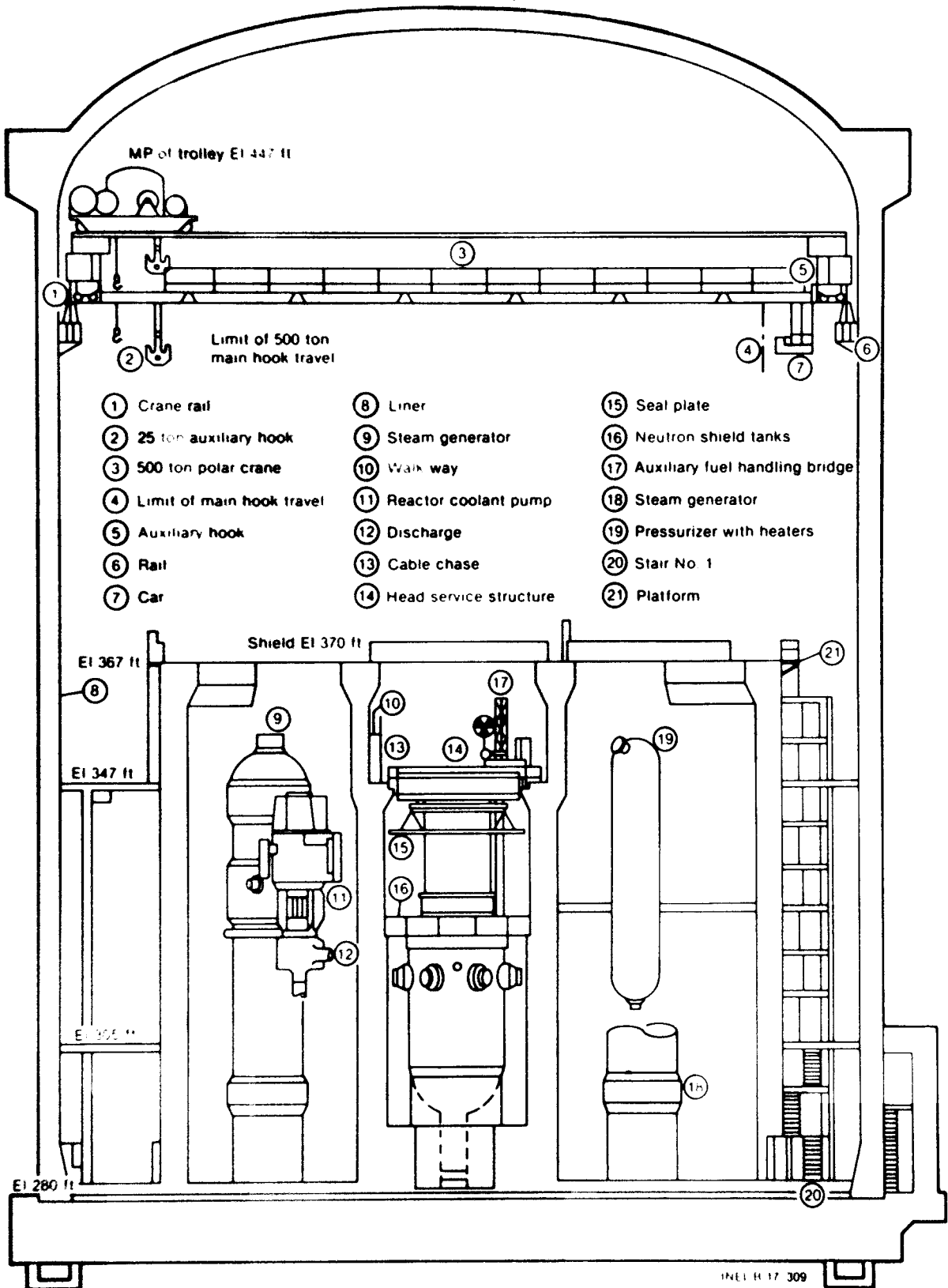
Figure 1. Cross section of the TMI-2 Reactor Containment Building.
