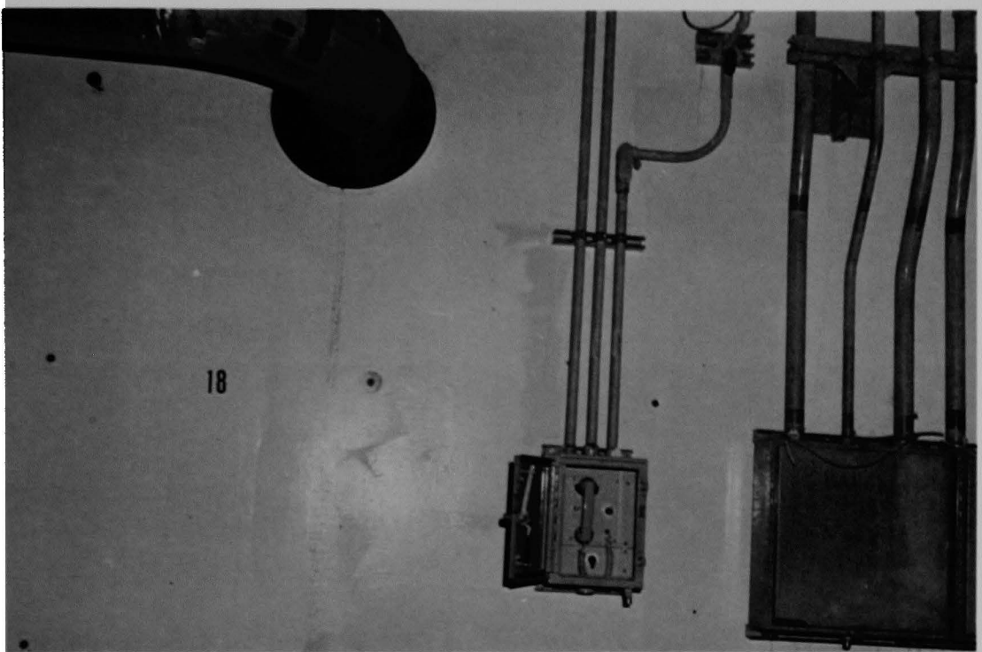
Figure 64 (2A). Core flood tank inlet piping, Gai-tronic telephone, and source range instrumentation panel.
