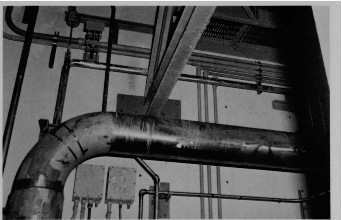
Figure 61 (2A). Core flood tank B piping running under access platform to core flood tank valves.
