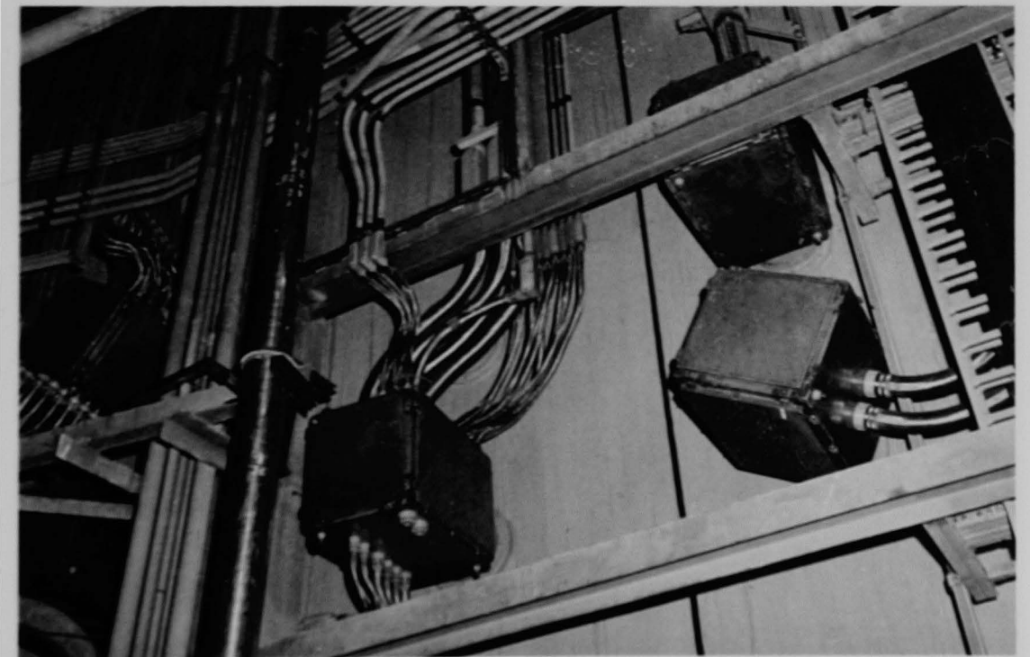
Figure 75 (5A). Electrical penetrations on containment liner; R-504 top, R-505 left, R-507 center right.
