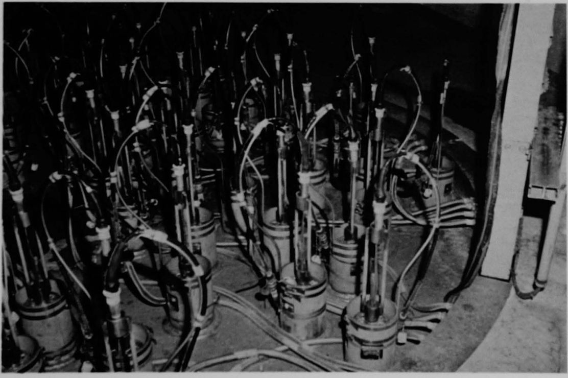
Figure 180 (4A). West side of the incore seal table. (This photograph was taken to document boron crystal accumulation.)
