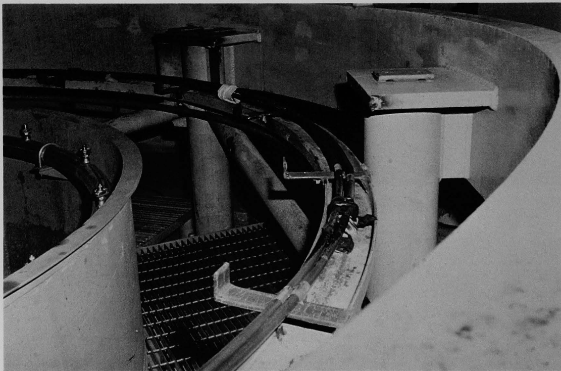
Figure 157 (6A). View inside of the head storage stand, looking west (tops of vessel guide studs appearing above rim); stainless steel spray line left.
