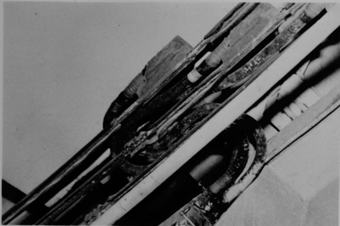
Figure 280 (5B). Close-up of power and controller buss bars for the polar crane.
