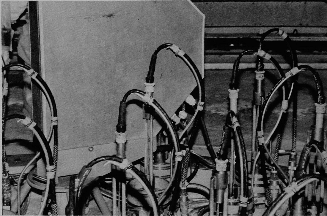
Figure 177 (4B). Incore instrumentation seal table (the metal cover houses the cable wheel for the movable incore detector. This photograph was taken to document boron crystal accumulation.)
