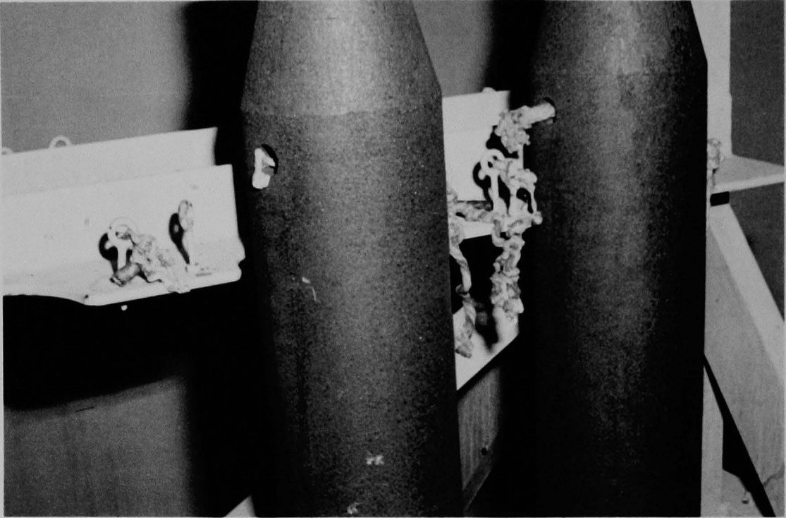
Figure 152 (4 ). Close-up of reactor vessel guide studs and melted rod rope.
