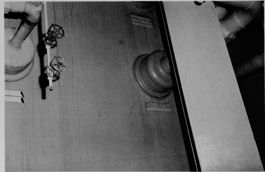
Figure 89 (5A). Mechanical penetrations on the containment wall; R-562, top center; R-559, R-563, and R-567 (left to right).
