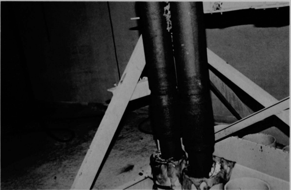
Figure 151 (2B). Reactor vessel guide studs.
