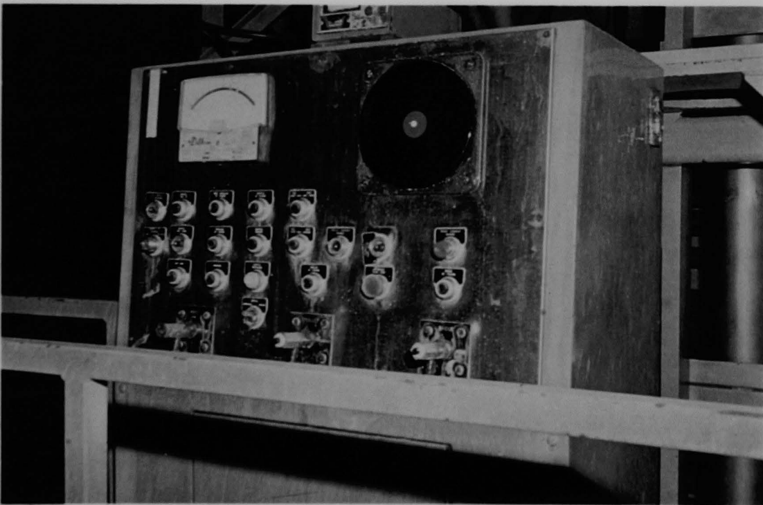
Figure 234 (6A). Operator's panel on the auxiliary fuel handling bridge, second or closer view.
