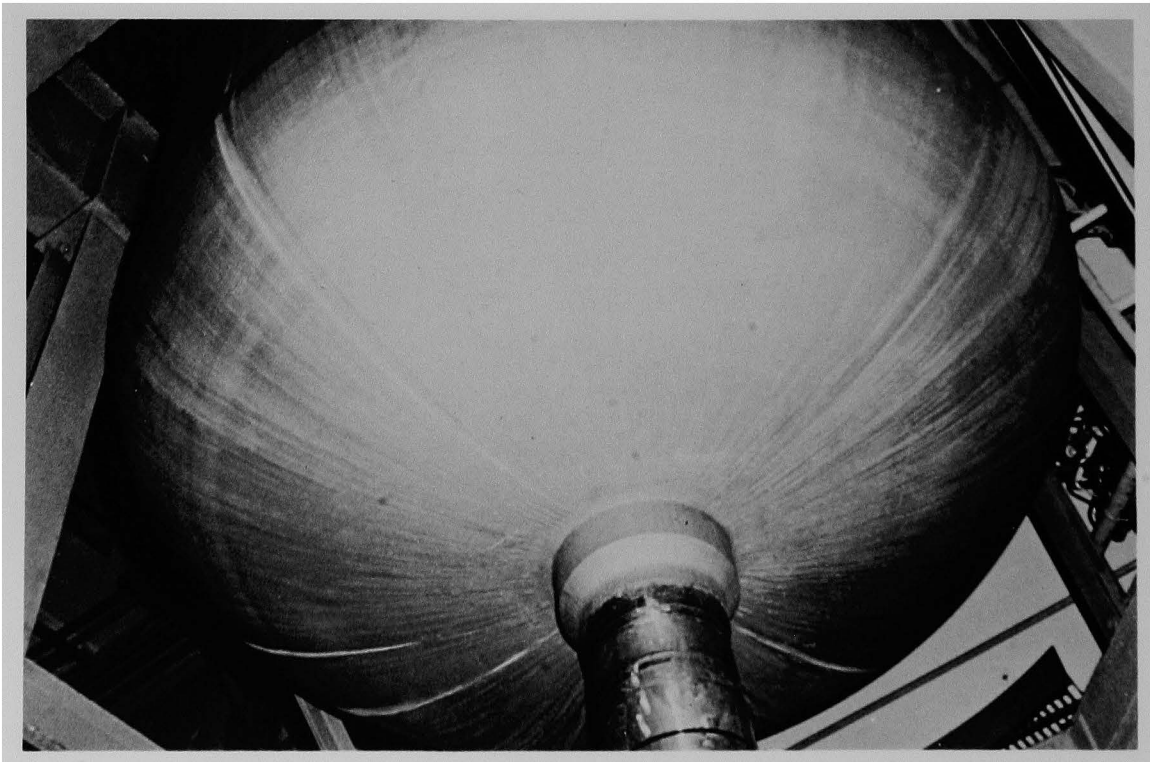
Figure 63 (1A). Bottom view of core flood tank B.
