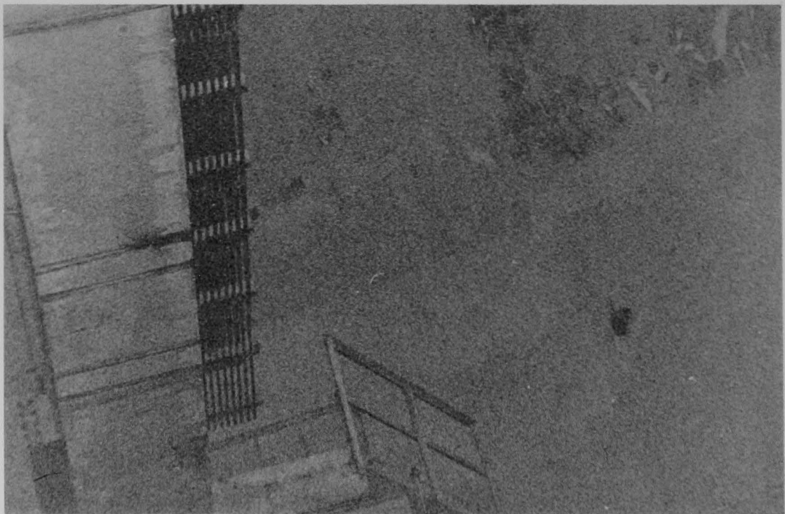
Figure 307 (5B). Northwest portion of girder B, showing trolley power and controller buss bars.
