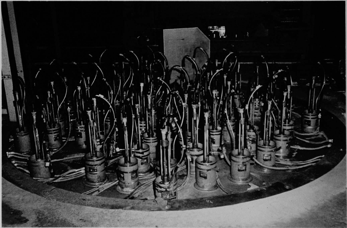
Figure 174 (4A). Incore instrumentation electrical connections; main fuel handling bridge background. (This photograph was taken to document boron crystal accumulation.)
