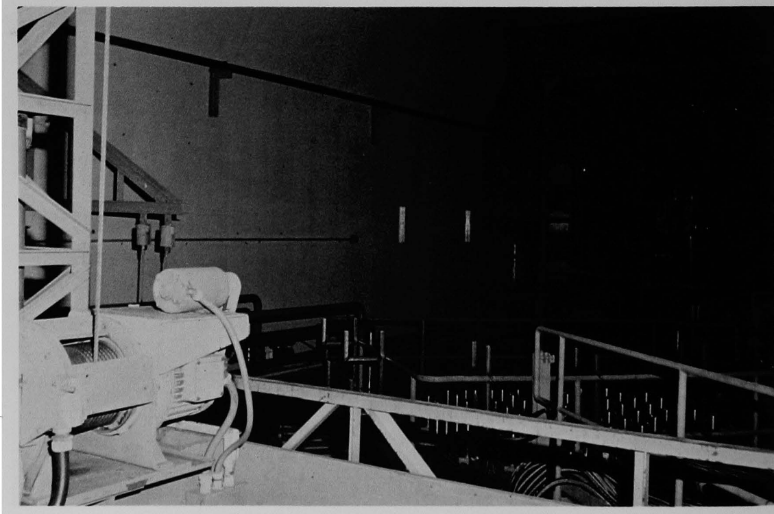
Figure 240 (2A). Top of the control rod drive mechanism (CRDM) platform above the reactor vessel; auxiliary fueling handling bridge foreground, main fuel handling bridge background right, first view.
