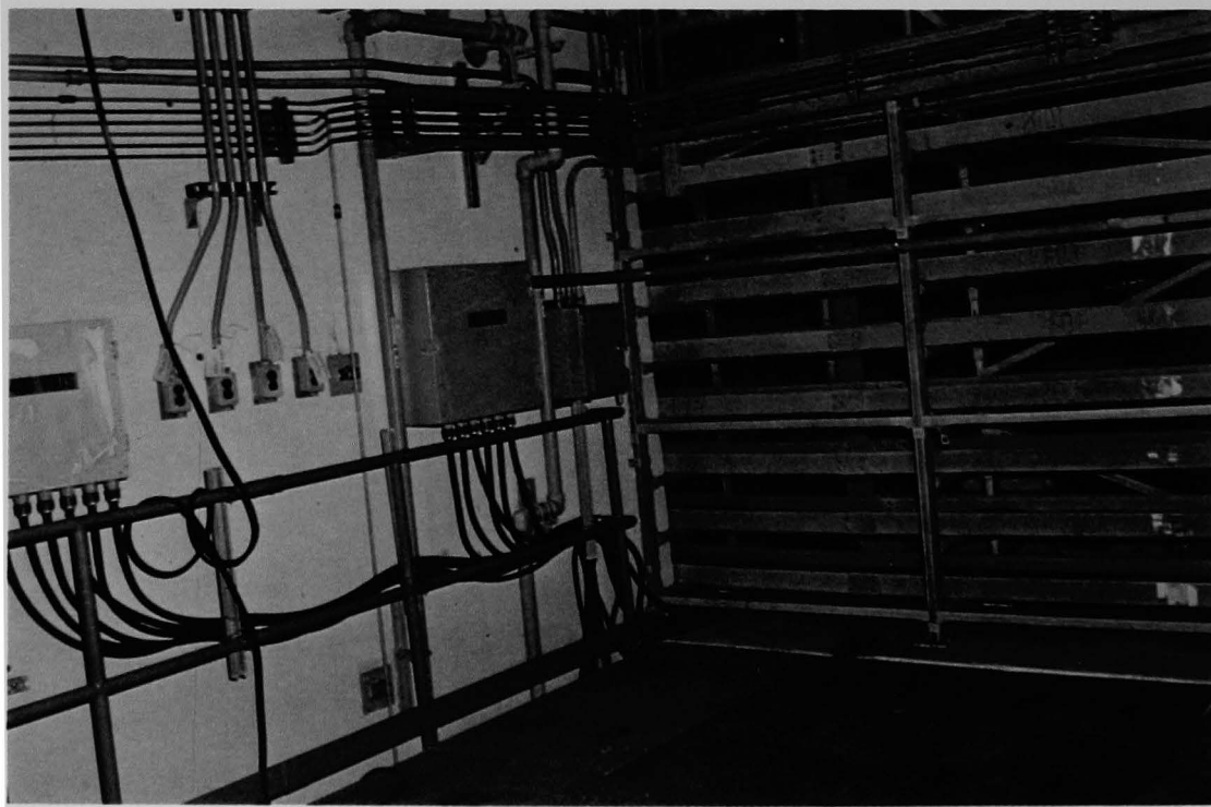
Figure 199 (4A). Energized electrical outlets and cable trays.
