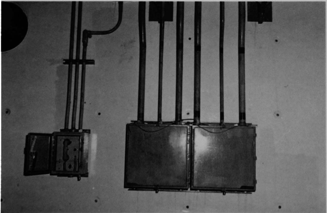
Figure 65 (2A). Gai-tronic telephone and source range instrumentation panel.
