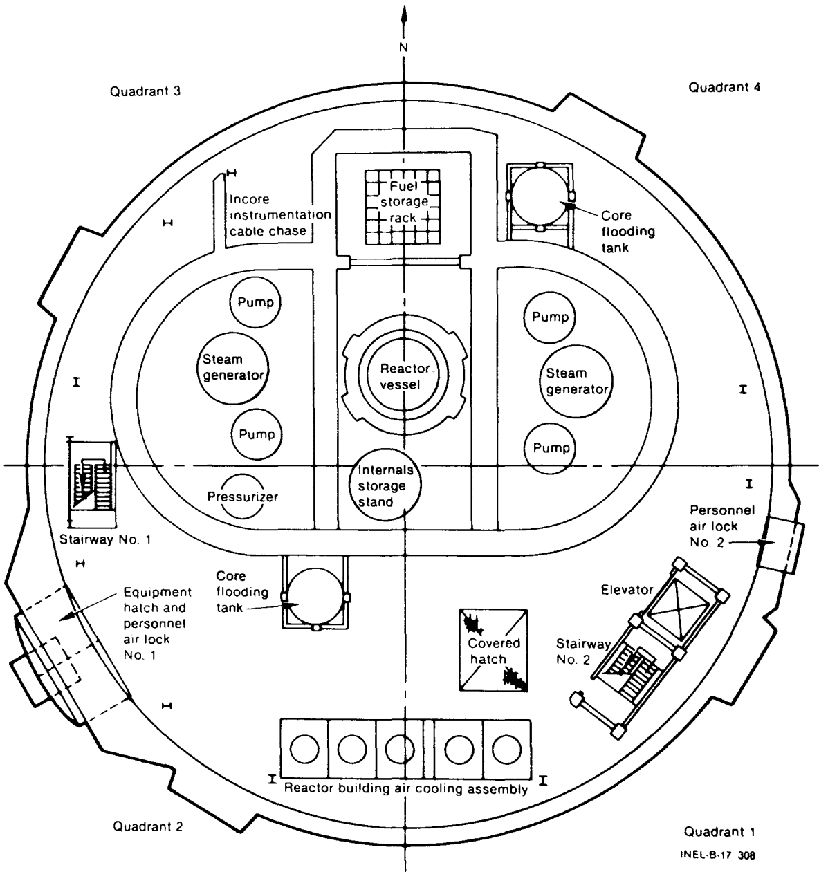
Figure ii. Floor plan of elevation 305, by quadrants.
