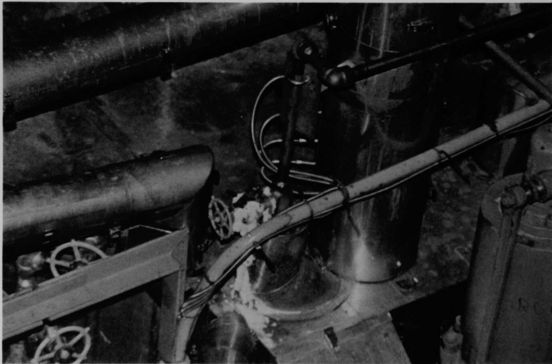
Figure 208 (4B). Valves and pipes above pressurizer (cf. Figure 178). The photograph was taken to document boron crystal accumulation.
