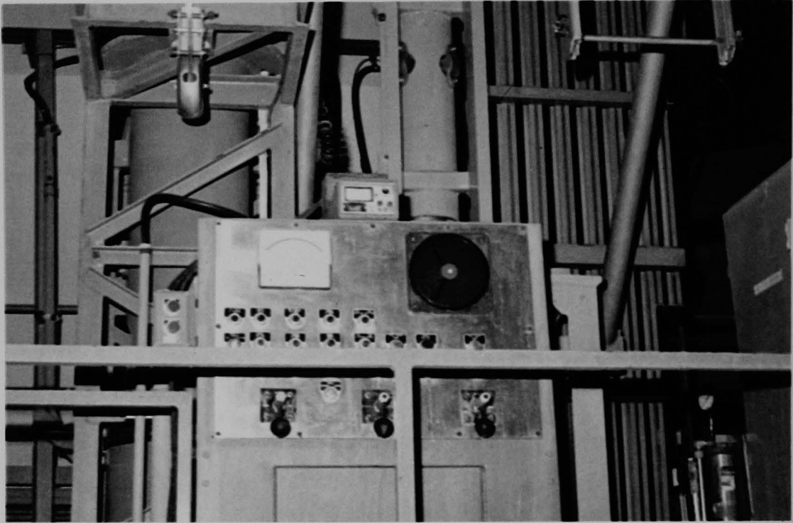
Figure 231 (4 ). Operator's panel on the auxiliary fuel handling bridge.
