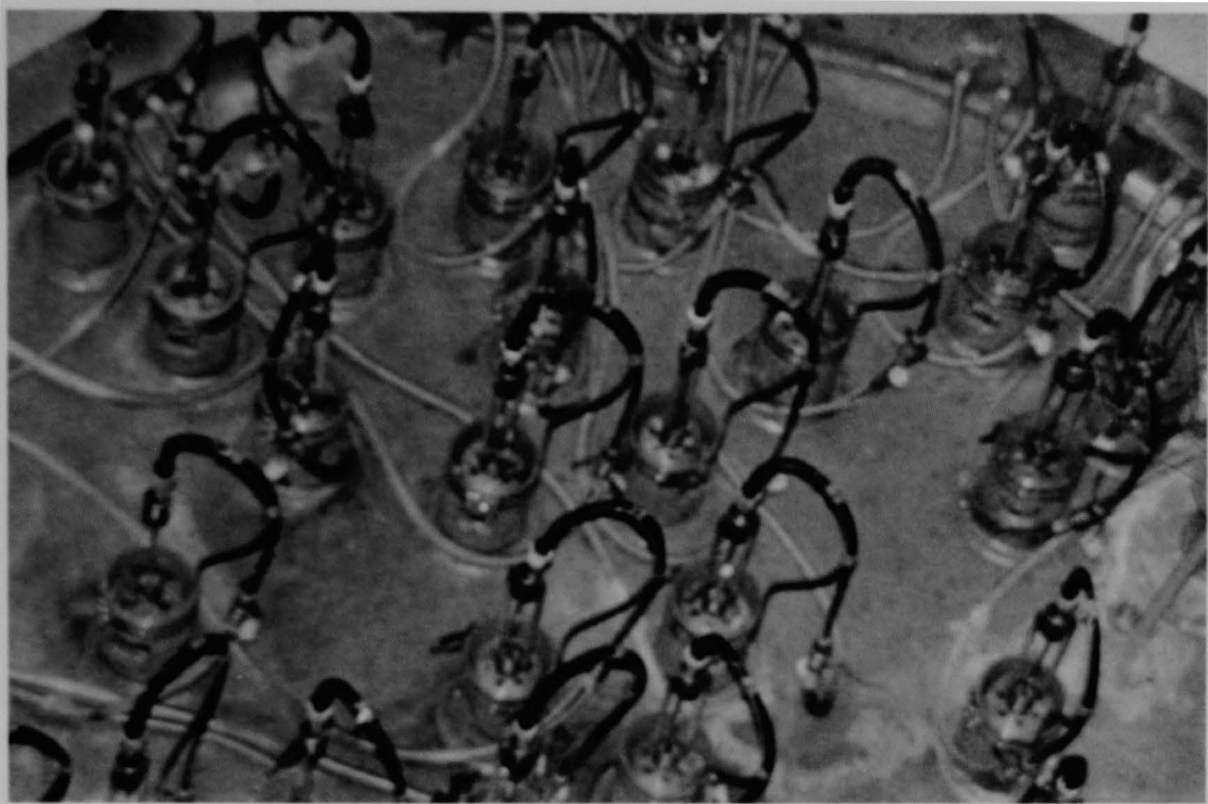
Figure 179 (4B). Incore seal table, view from above. (This photograph was taken to document boron crystal accumulation.)
