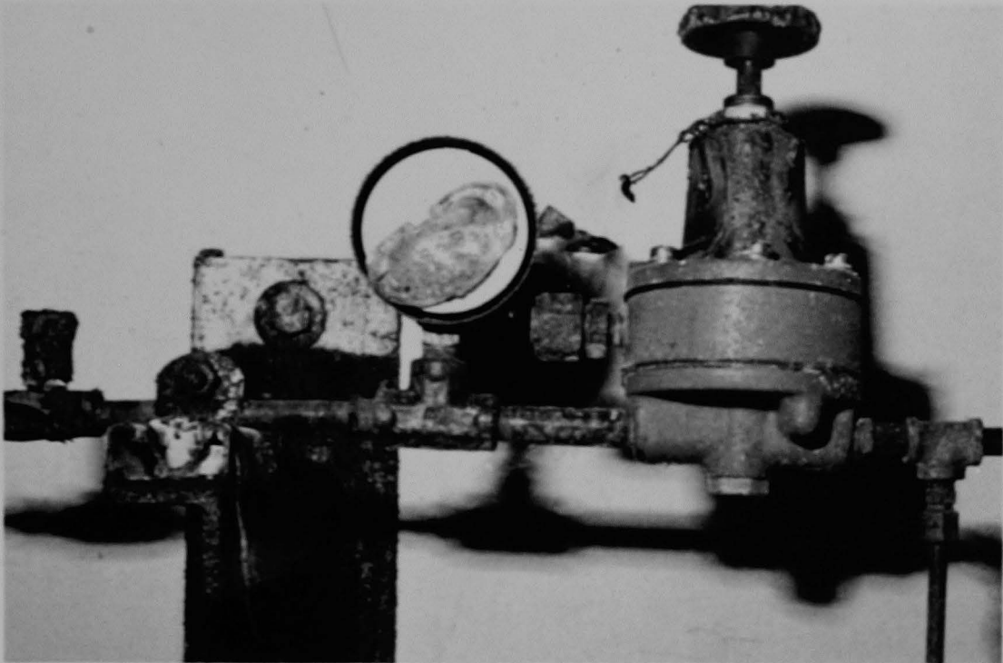
Figure 188 (4 ). Air pressure regulator mounted on the D-ring wall (see Figure 210) and a guage on which the lens has melted.
