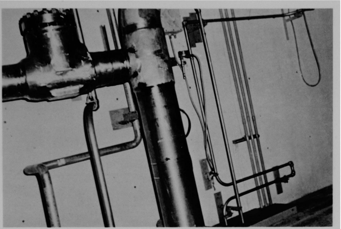
Figure 60 (1A). Core flood tank B piping on seismic support.
