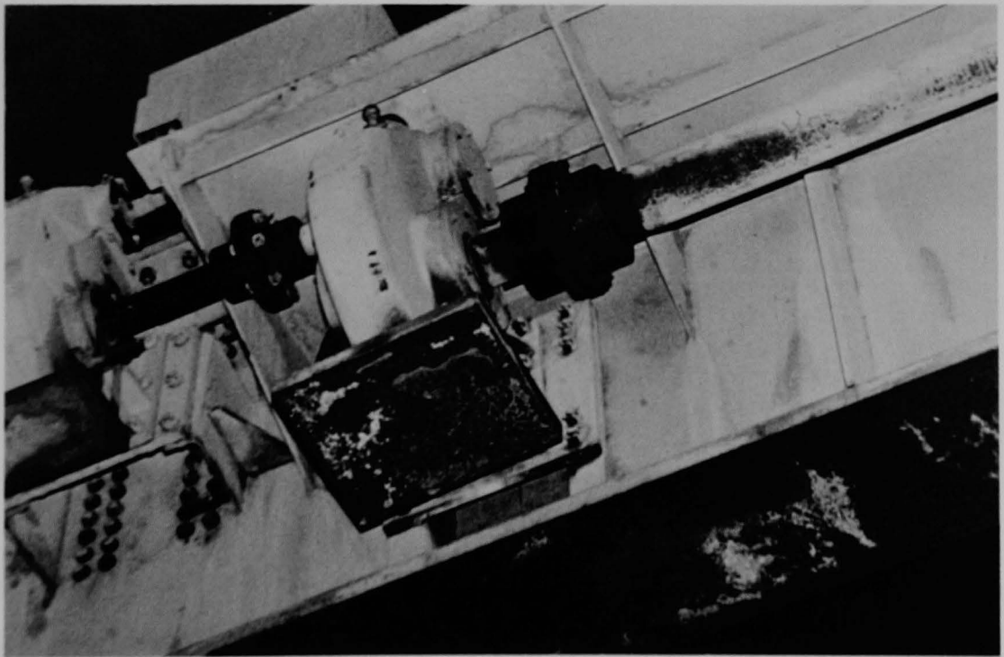
Figure 301 (5B). Gear housings and drive shafts on the trolley of the polar crane.
