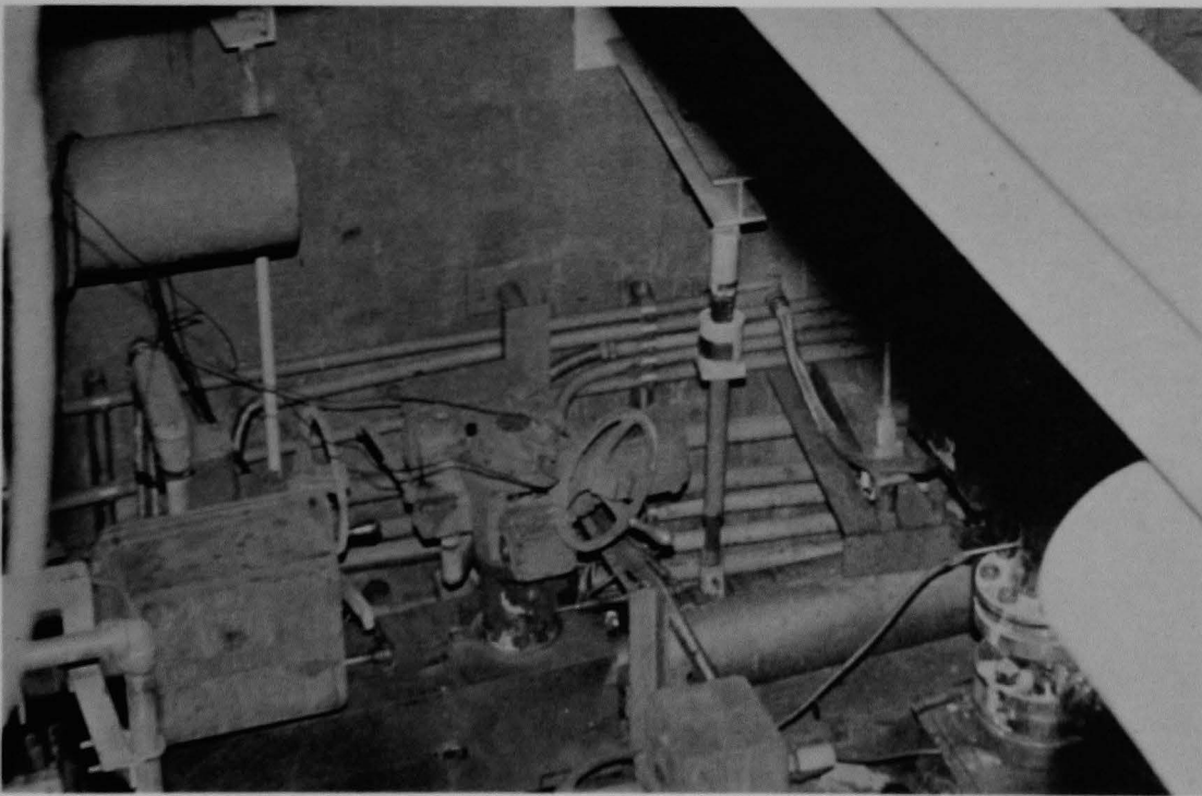
Figure 210 (4B). Pressure-operated release valve above the pressurizer. (The photograph was taken to document boron crystal accumulation).
