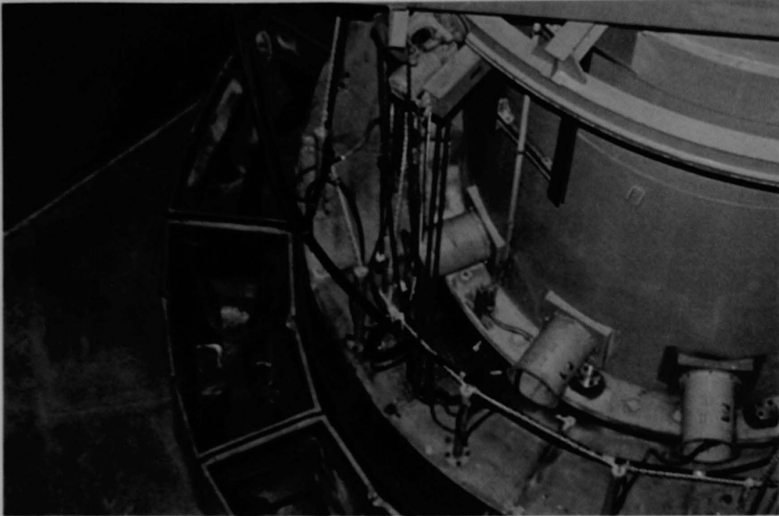
Figure 253 (4B). The reactor head from above (the neutron shield tanks appear to be dry).
