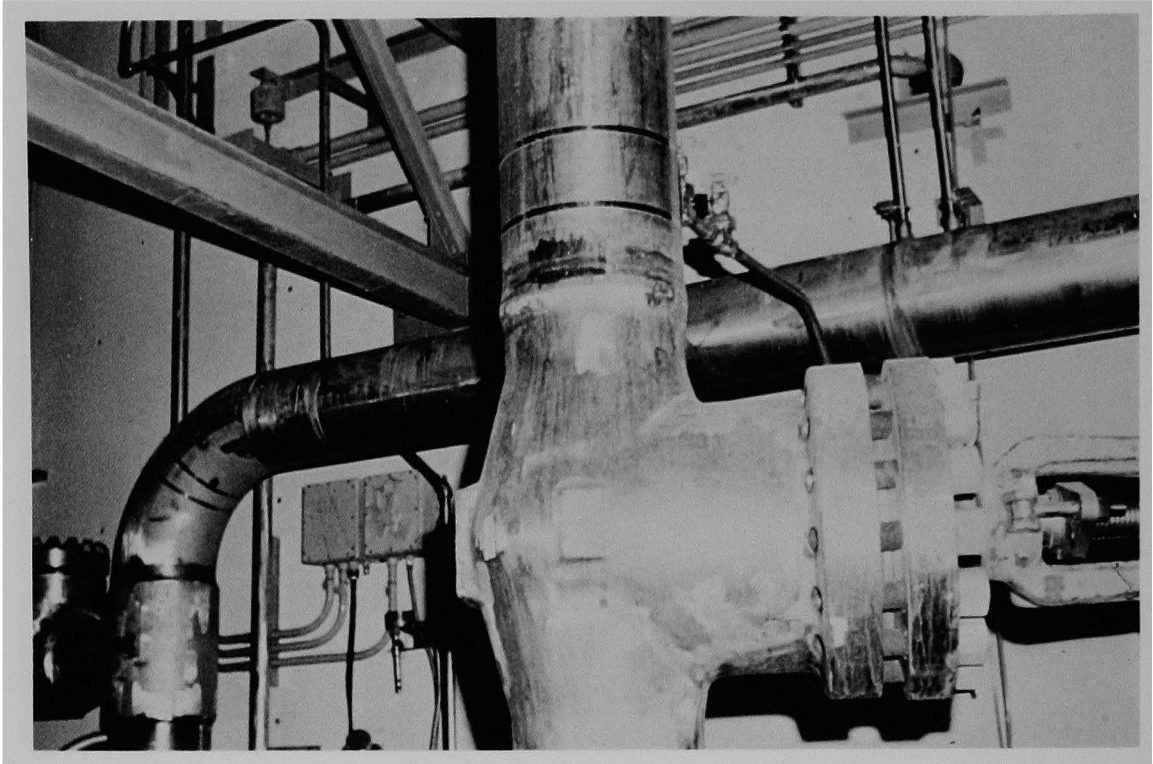
Figure 62 (1A). Check valve directly under core flood tank B.
