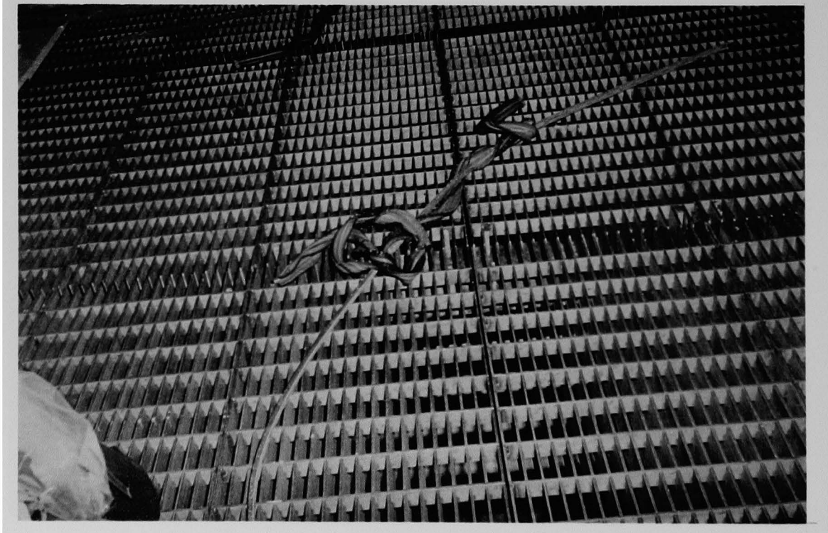
Figure 169 (4A). Polar crane power cable and insulation on grating over core flood tank B.
