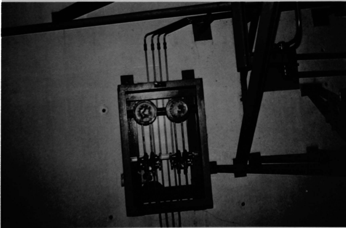
Figure 83 (2B). Gauges and instrumentation along northeast side of D-ring.
