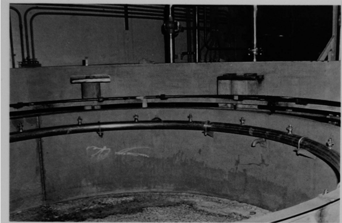
Figure 158 (6A). Northeast view inside of the head storage stand at stainless steel spray line used to decontaminate the reactor head.
