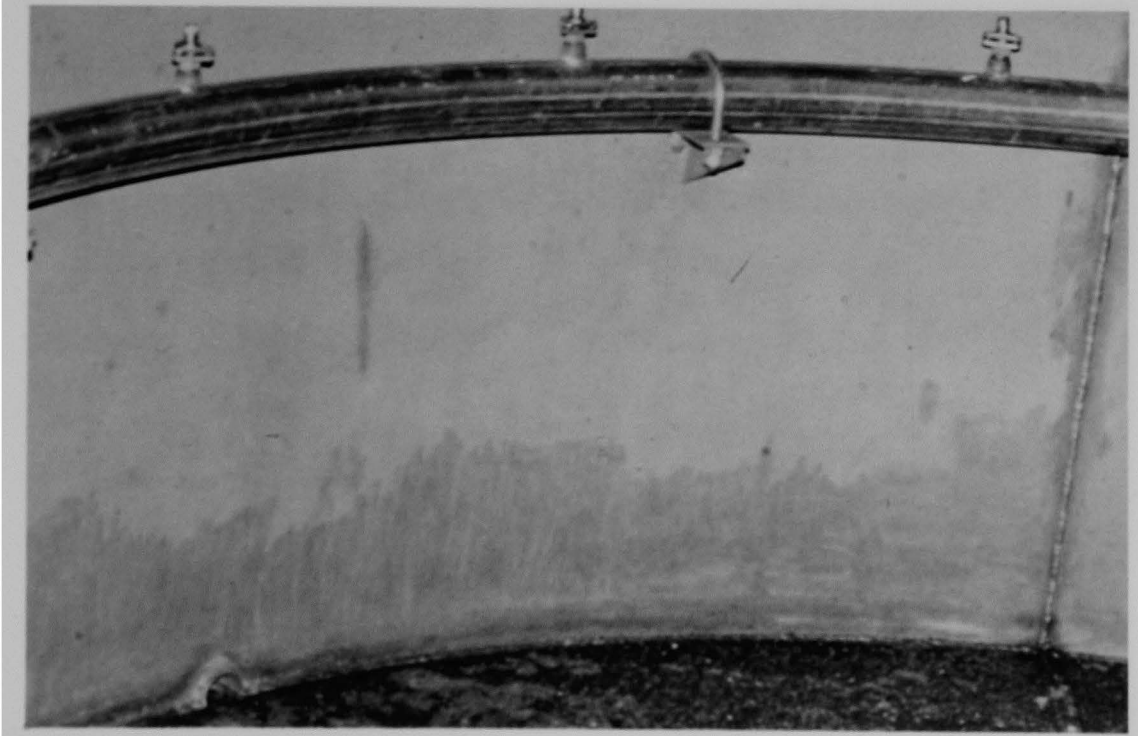
Figure 159 (4B). Section of the stainless steel spray line inside of the head storage stand.
