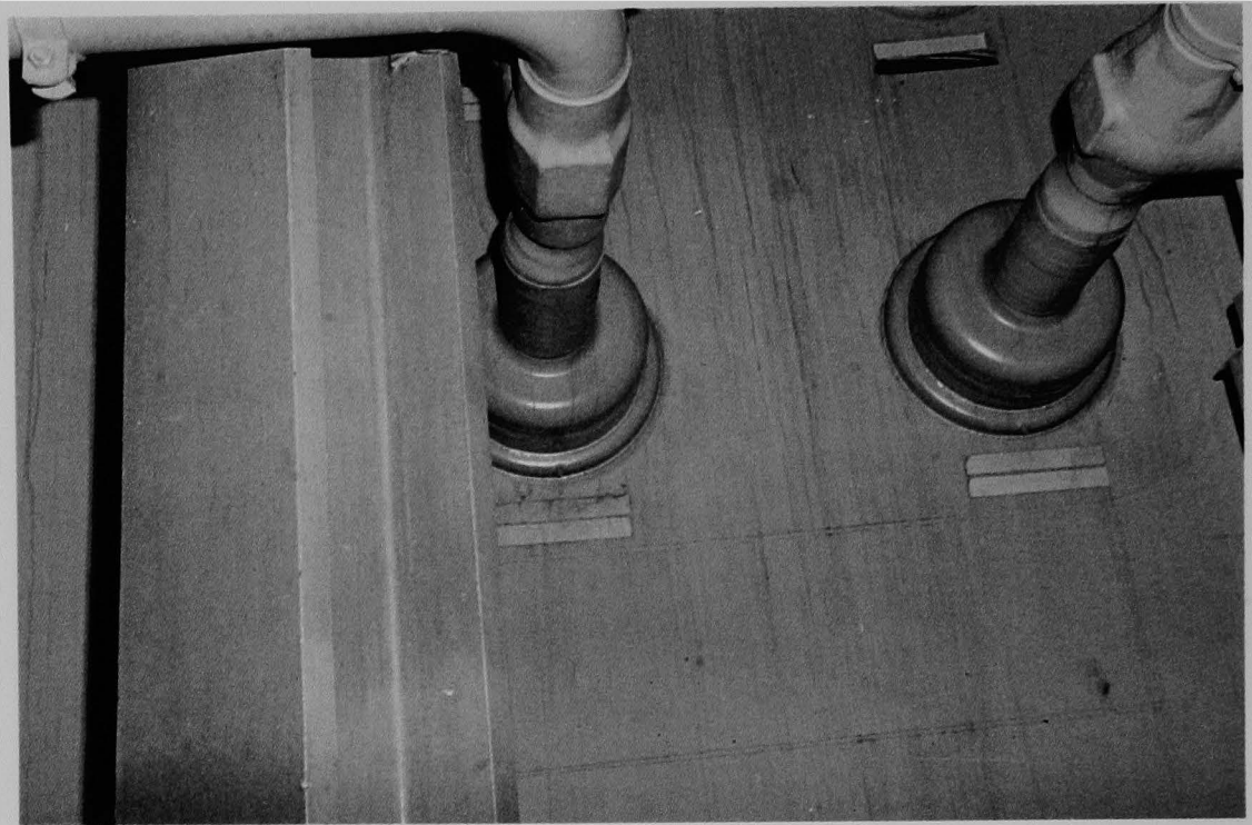
Figure 88 (5A). Mechanical penetrations R-563 and R-567, second view.
