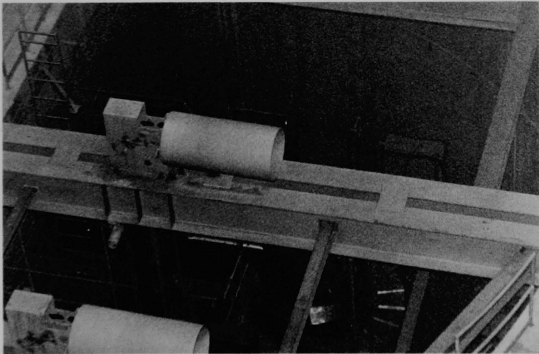
Figure 220 (5B). View down into D-ring B showing seismic support for equipment.
