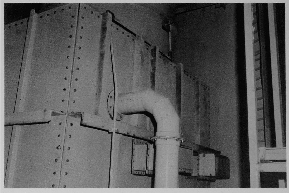
Figure 47 (6A). Plenum at upper west end of air cooling assembly.
