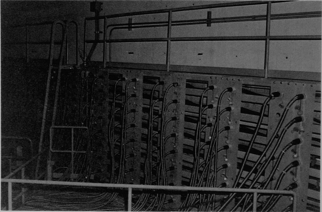
Figure 247 (6A). CRDM cable trays along D-ring B; walkway above, access ladder left.
