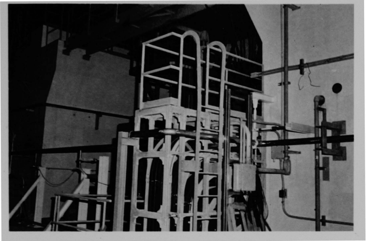
Figure 129 (2A). Control rod drive mechanism cable trays (see Figure 97, left).
