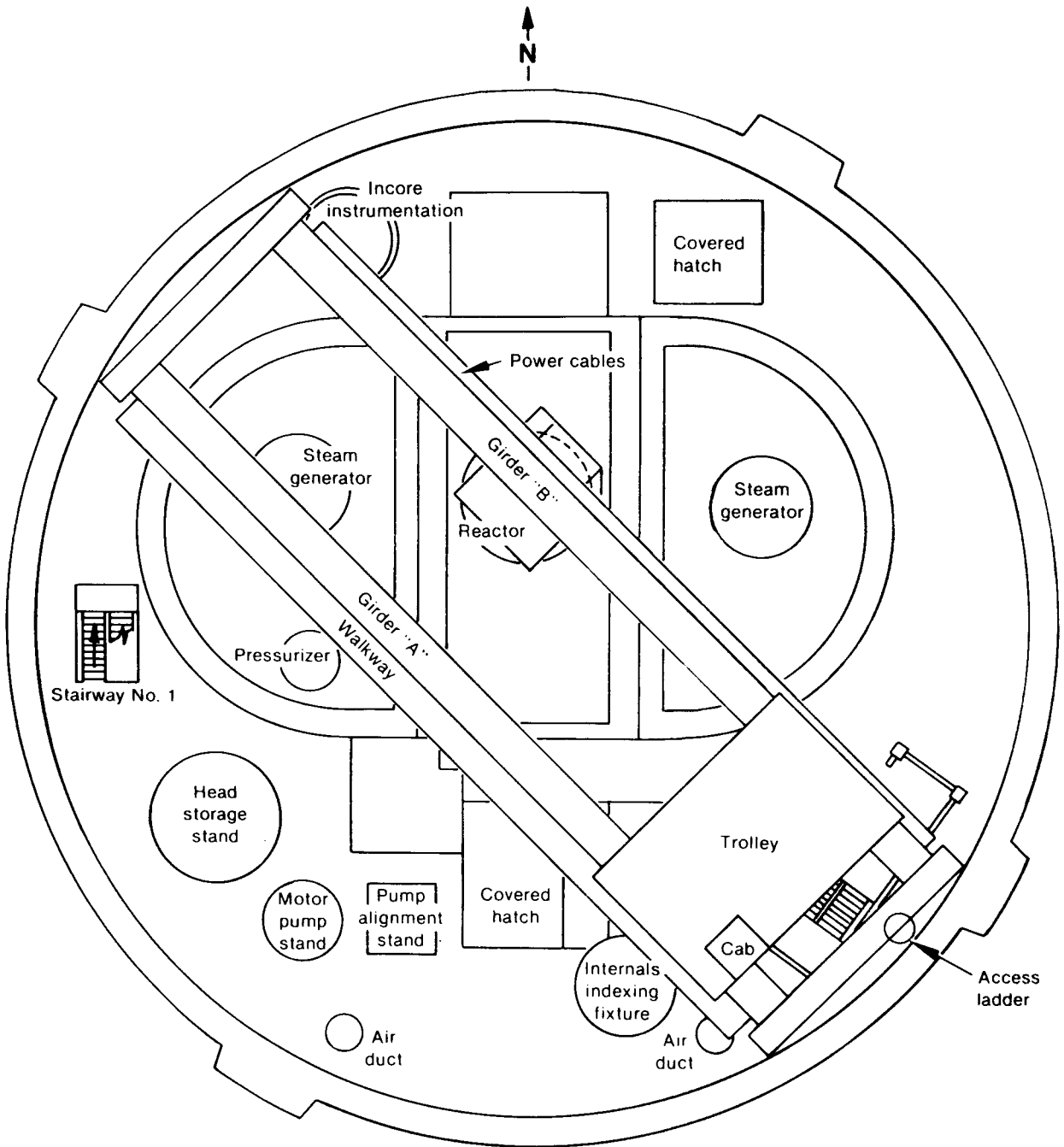
Figure iv. Floor plan of elevation 347, with polar crane superimposed.
