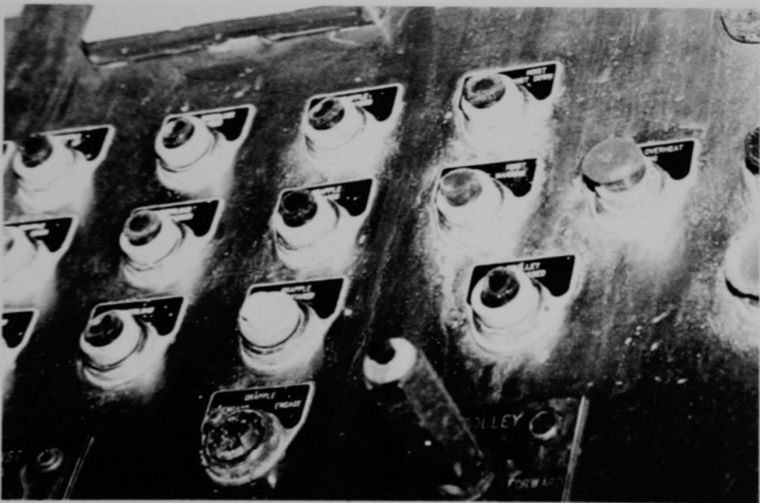
Figure 238 (5B). Close-up of the control panel on the auxiliary fuel handling bridge, third view.
