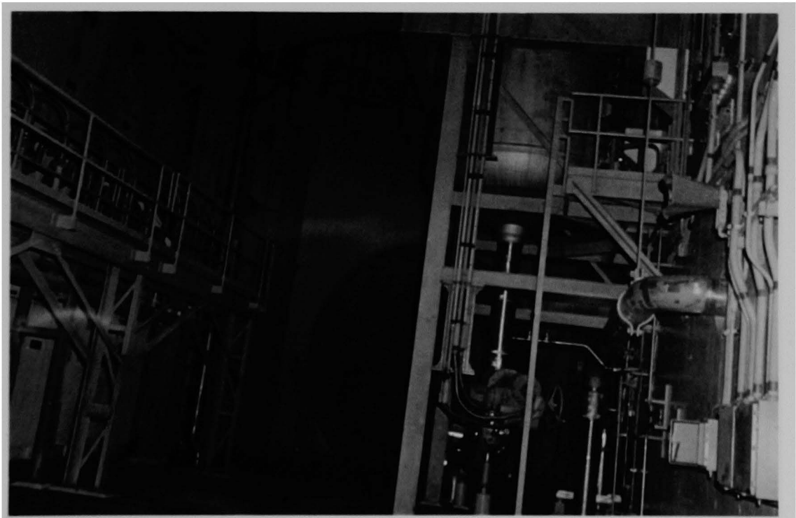
Figure 49 (2A). From left: air coolers, personnel air lock 1 within equipment hatch, core flood tank B, D-ring wall.
