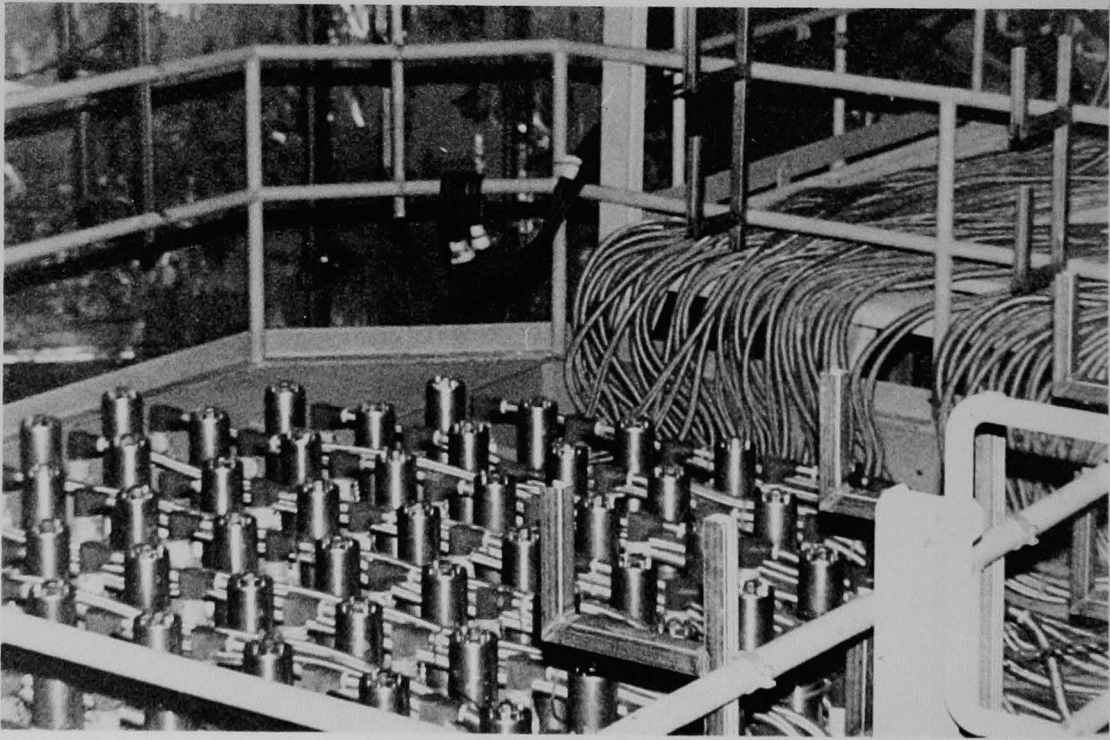
Figure 248 (5B). Close-up of the CRDM platform above the reactor vessel.
