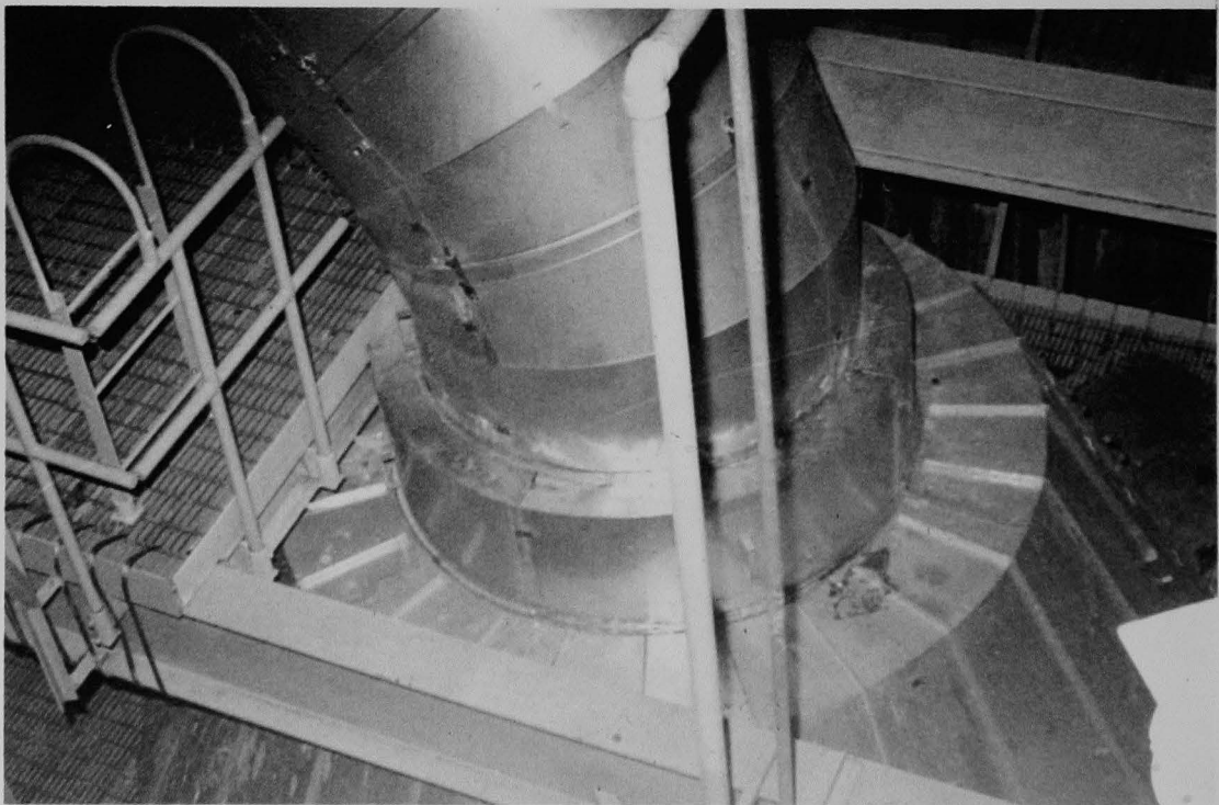
Figure 212 (4 ). Top of steam generator A from northwest.
