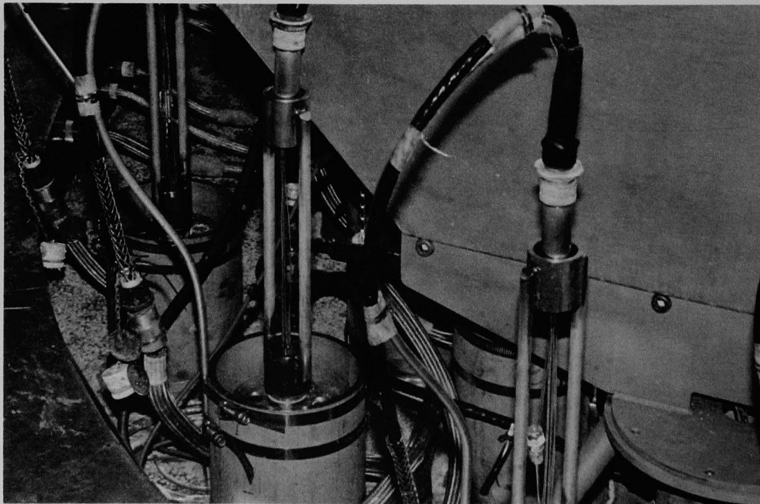
Figure 178 (4B). Incore instrumentation seal table, closer view and taken from behind metal box (cf. Figure 190).
